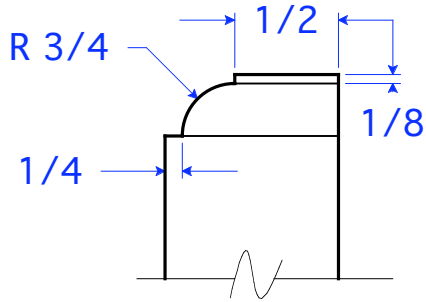
BM 14-1.5 Profile Not To Scale
