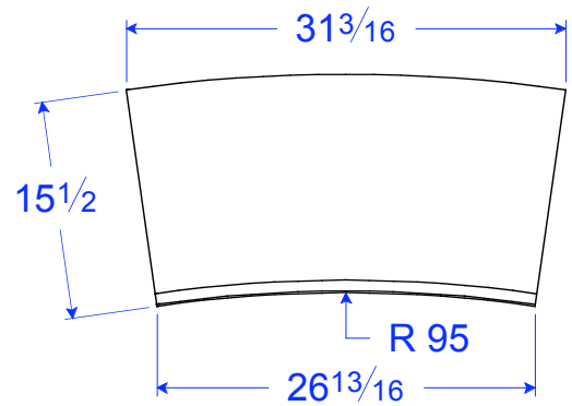
BM 14-1.5x15.5 STR R95 15 1/2"H x 31 3/16"L x 1 1/2"T
