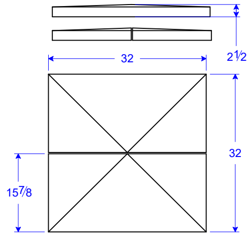
PC 13-16 P2.5* 15 7/8W x 32L x 2.5H * Two Pieces Needed To Make A Pier Cap 32 x 32 x 2.5
