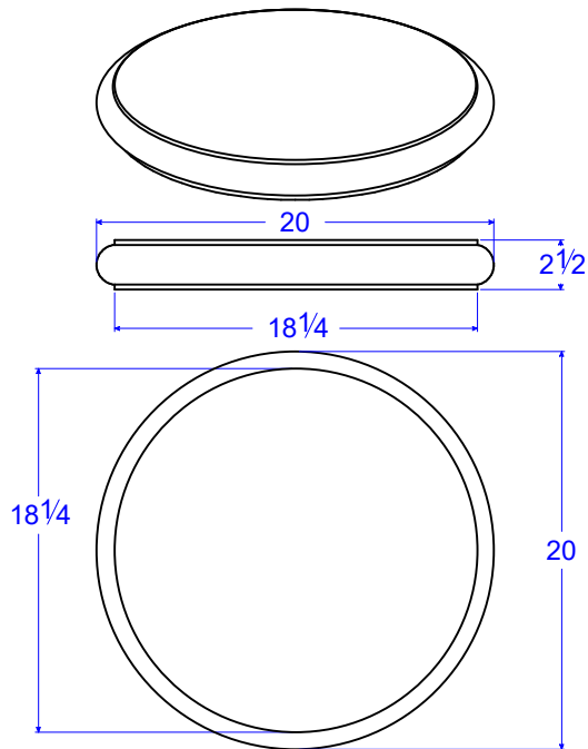
PC 31-22 BN RD F 20" Dia. x 2 1/2"H
