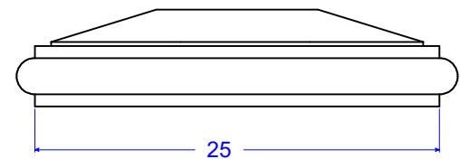
PC 31-27.25 x 21.25 BN P6 19"W x 25"L x 6"H
