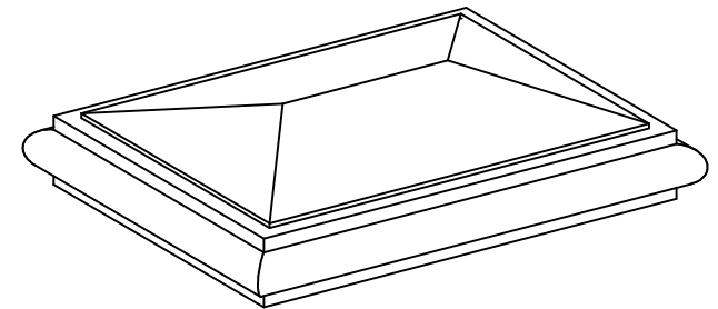
PC 31-19 BN P3.5 17"W x 17"L x 3 1/2"H
