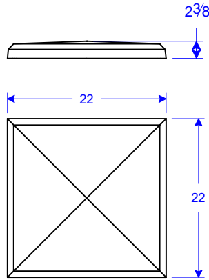
PC 40-22 BV P2.375 22"W x 22"L x 2 3/4"H
