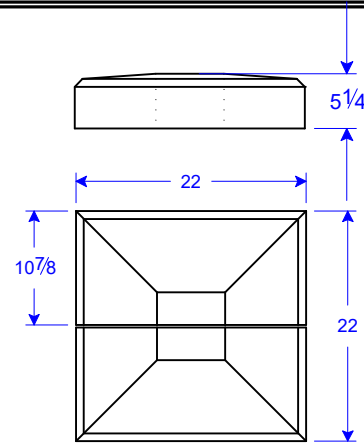
PC 40-22 Split BV P5.25 10 7/8"W x 22"L x 5 1/4"H
