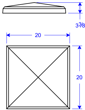
PC 40-20 BV P 3 3/8 20"W x 20"L x 3 3/8"H
