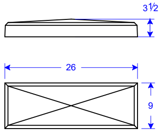
PC 40-9 BV P 3.5 9"W x 26"L x 3 1/2"H
