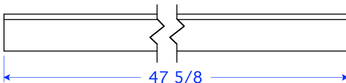
SM 27-7.625x3.5:3 STR 7 5/8"W x 47 5/8"L x 3 1/2"H
