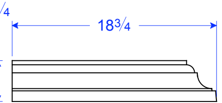
TM 26-2 RR 4 3/4"W x 18 3/4"L x 3 3/4"H
