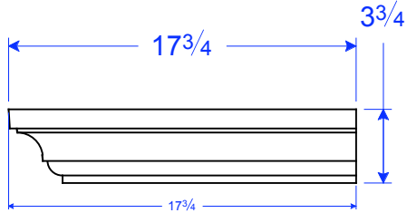
TM 26-2M LR 4 3/4"W x 17 3/4"L x 3 3/4"H
