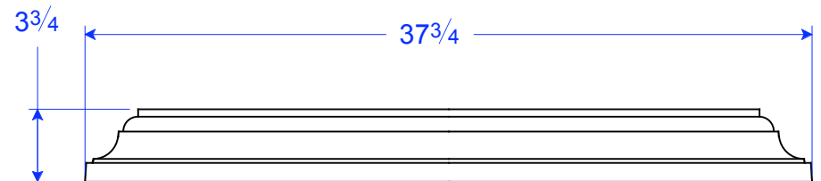
TM 26-2 DR 4 3/4"W x 37 3/4"L x 3 3/4"H
