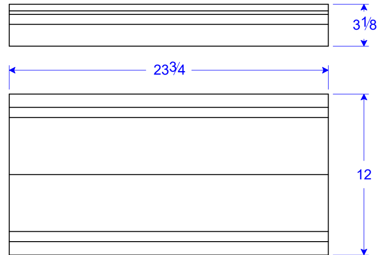
WC 19-12 STR 12"W x 23 3/4"L x 3 1/8"H
