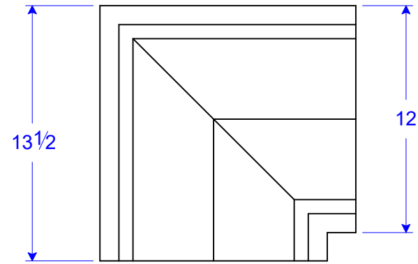
WC 19-12 CF 12"W x 13 1/2" Sq. x 3 1/8"H
